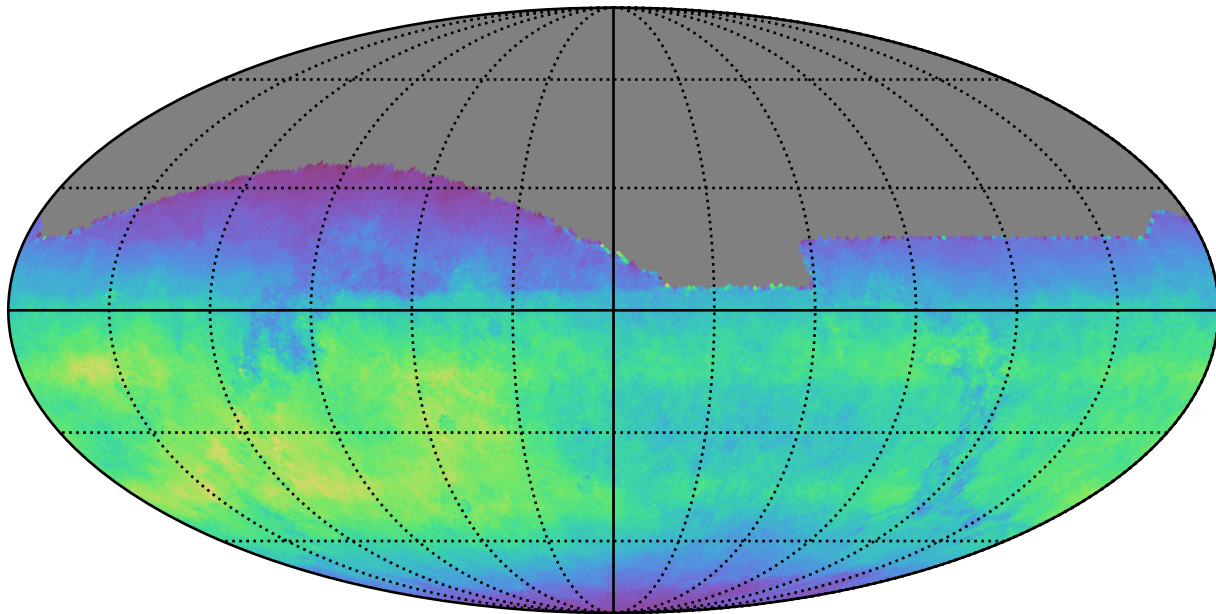
too_elab_r32_d3_giz_v3.4_10yrs All sky i band: Normalized Teff
