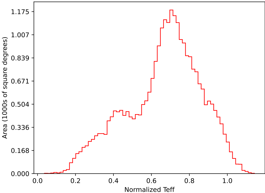
too_elab_r32_d3_giz_v3.4_10yrs All sky i band: Normalized Teff
