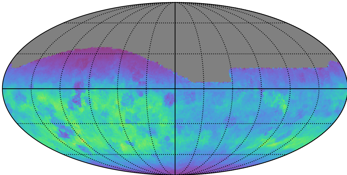
too_elab_r32_d3_giz_v3.4_10yrs All sky g band: Normalized Teff
