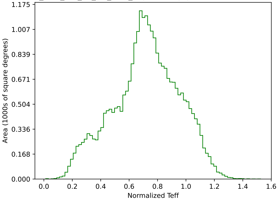
too_elab_r32_d3_giz_v3.4_10yrs All sky g band: Normalized Teff
