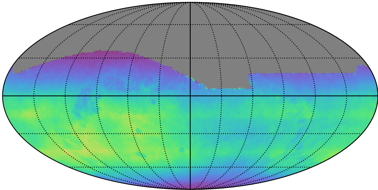
too_elab_r32_d3_giz_v3.4_10yrs All sky all bands: Normalized Teff
