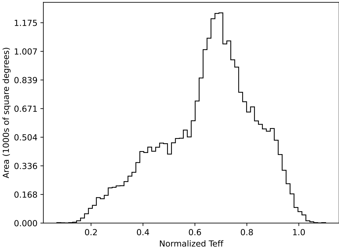
too_elab_r32_d3_giz_v3.4_10yrs All sky all bands: Normalized Teff
