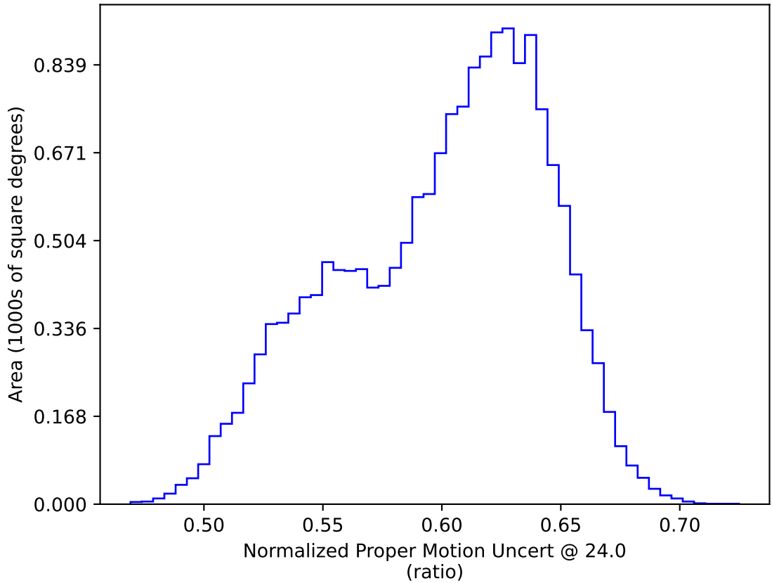
too_elab_r32_d3_giz_v3.4_10yrs WFD: Normalized Proper Motion Uncert @ 24.0
