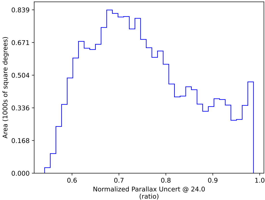
too_elab_r32_d3_giz_v3.4_10yrs WFD: Normalized Parallax Uncert @ 24.0
