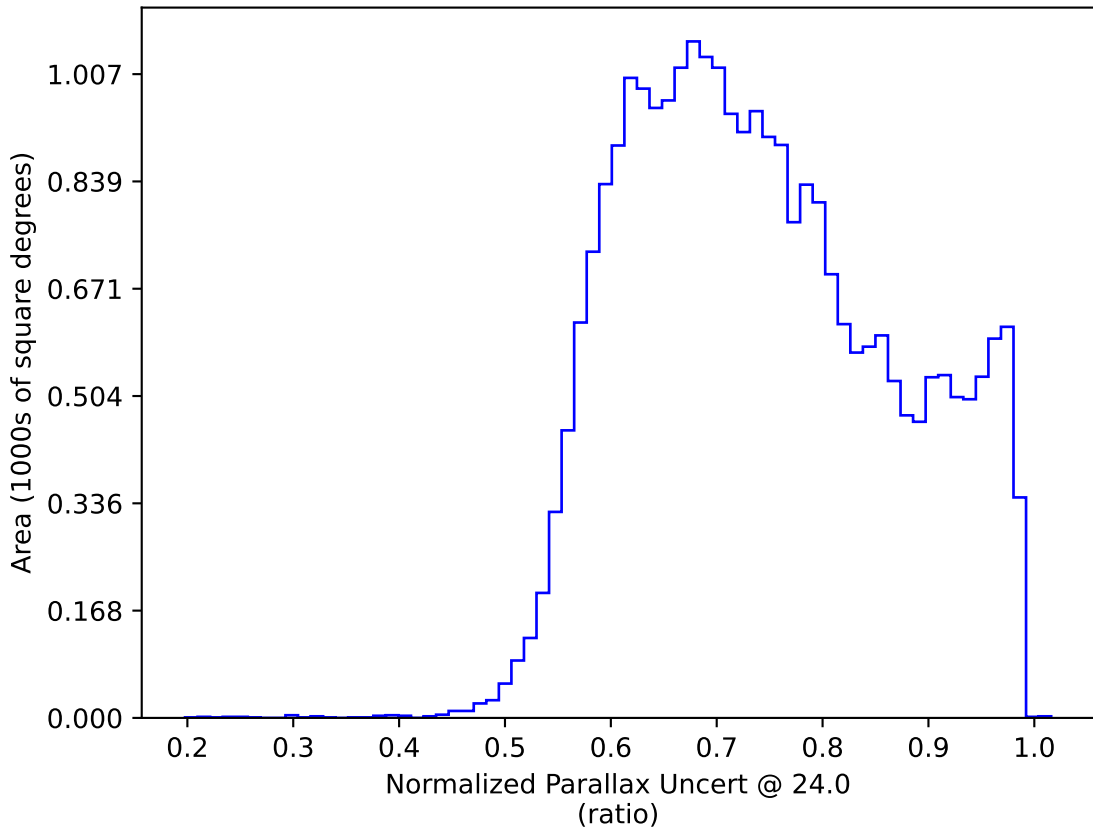
too_elab_r32_d3_giz_v3.4_10yrs All sky: Normalized Parallax Uncert @ 24.0
