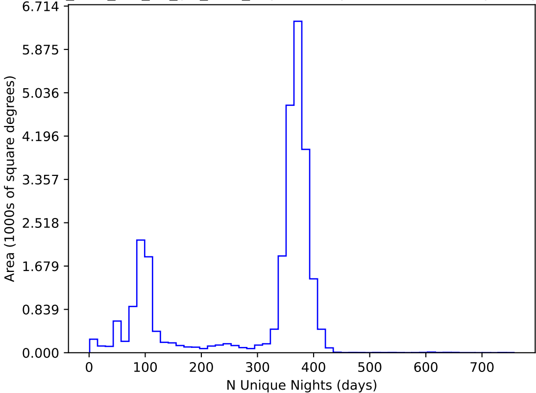
too_elab_r32_d3_giz_v3.4_10yrs All sky all bands: N Unique Nights
