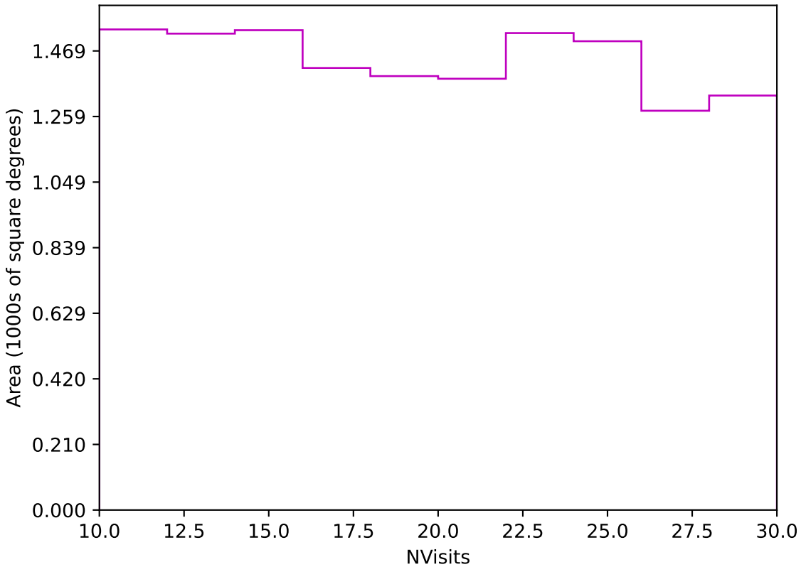
too_elab_r32_d3_giz_v3.4_10yrs Yr 3-4 z band: NVisits
