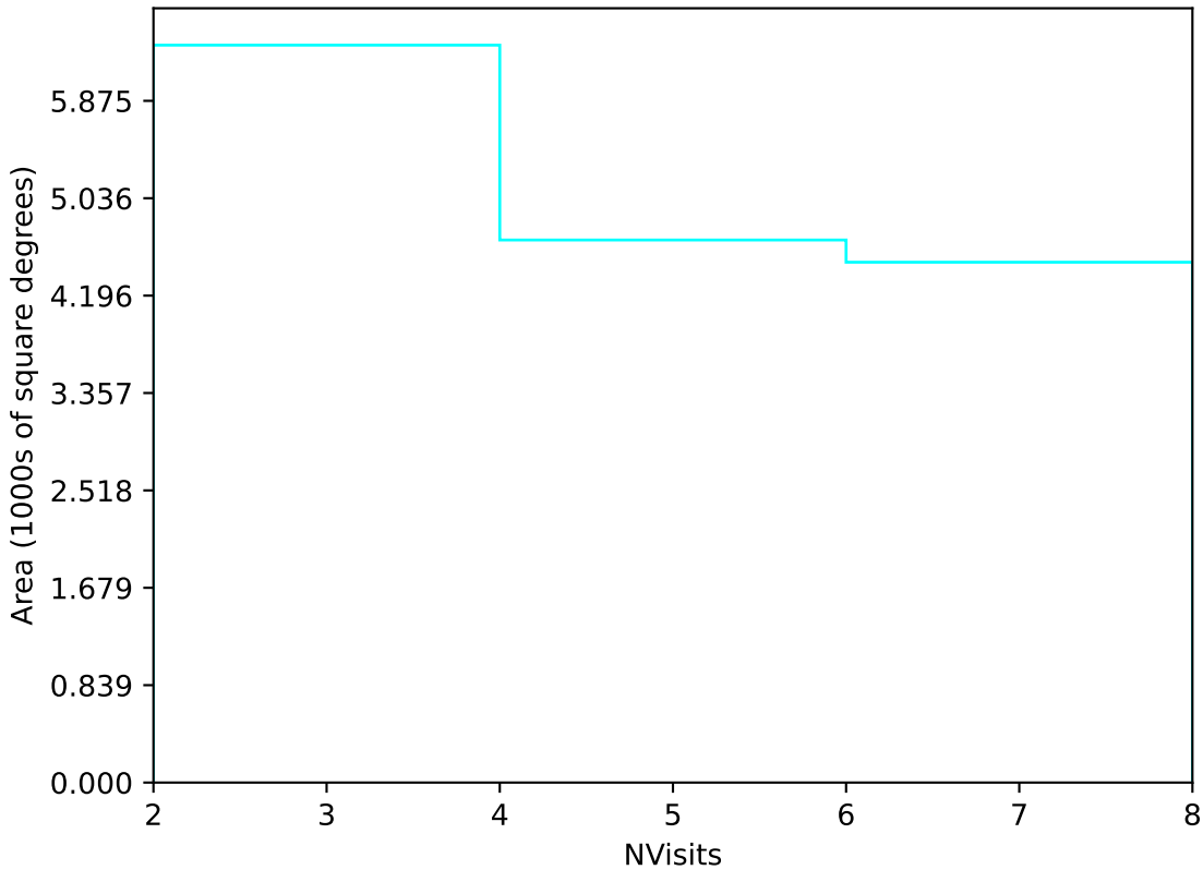
too_elab_r32_d3_giz_v3.4_10yrs Yr 3-4 u band: NVisits
