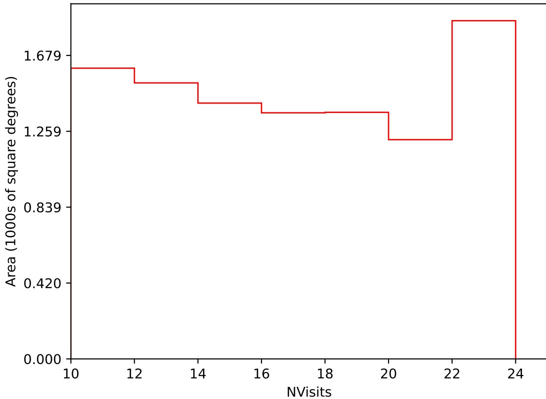
too_elab_r32_d3_giz_v3.4_10yrs Yr 3-4 i band: NVisits
