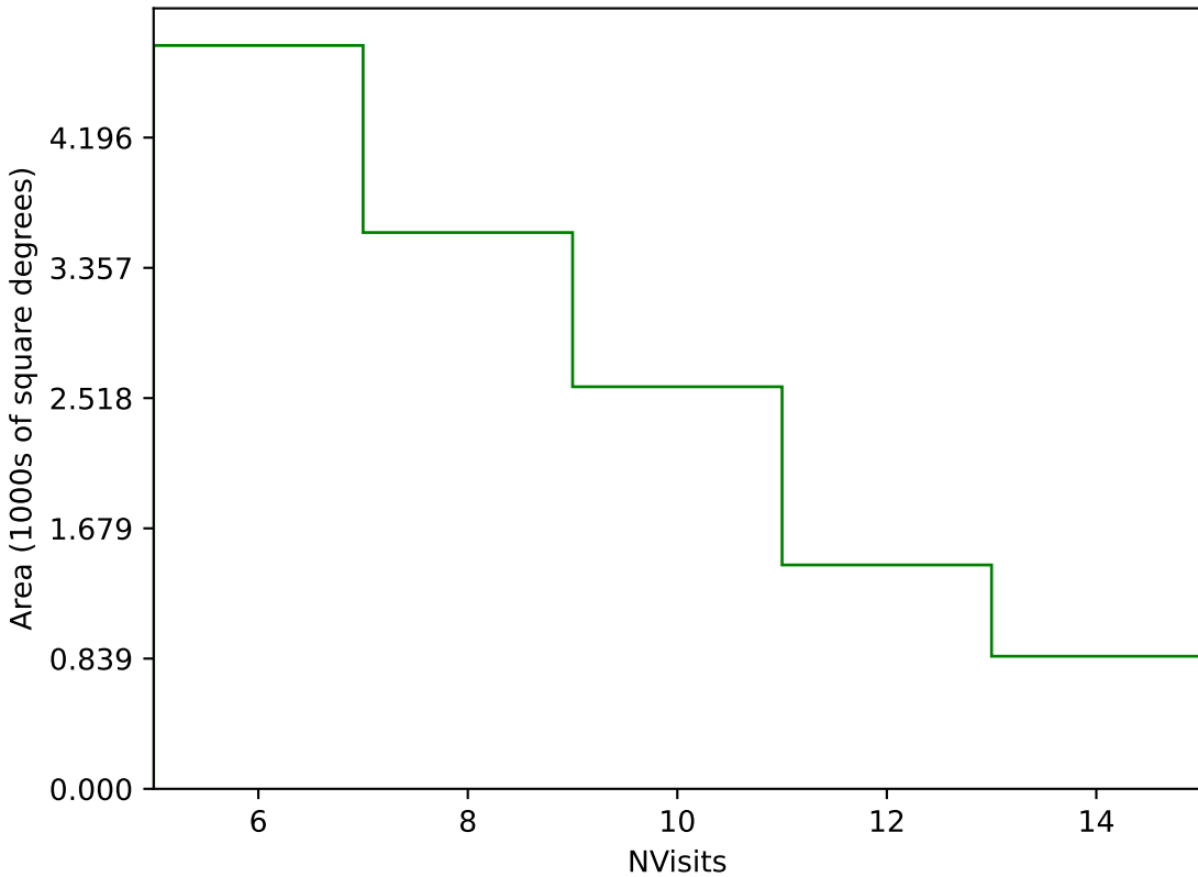
too_elab_r32_d3_giz_v3.4_10yrs Yr 3-4 g band: NVisits
