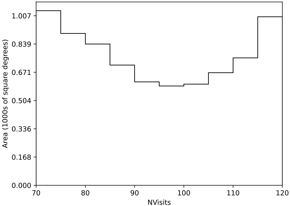
too_elab_r32_d3_giz_v3.4_10yrs Yr 3-4 all bands: NVisits
