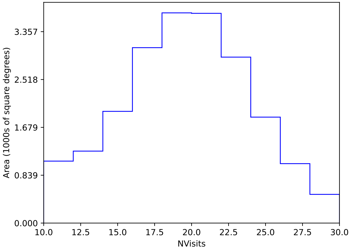
too_elab_r32_d3_giz_v3.4_10yrs Yr 1 y band: NVisits
