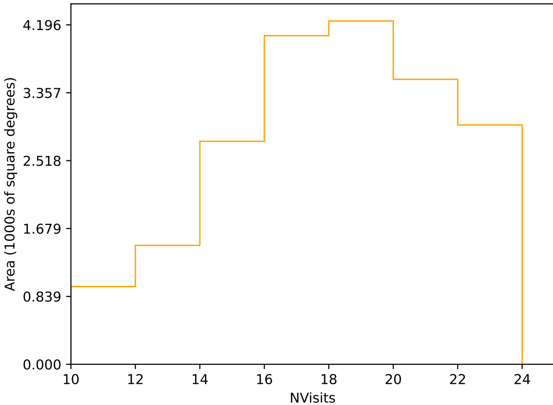
too_elab_r32_d3_giz_v3.4_10yrs Yr 1 r band: NVisits
