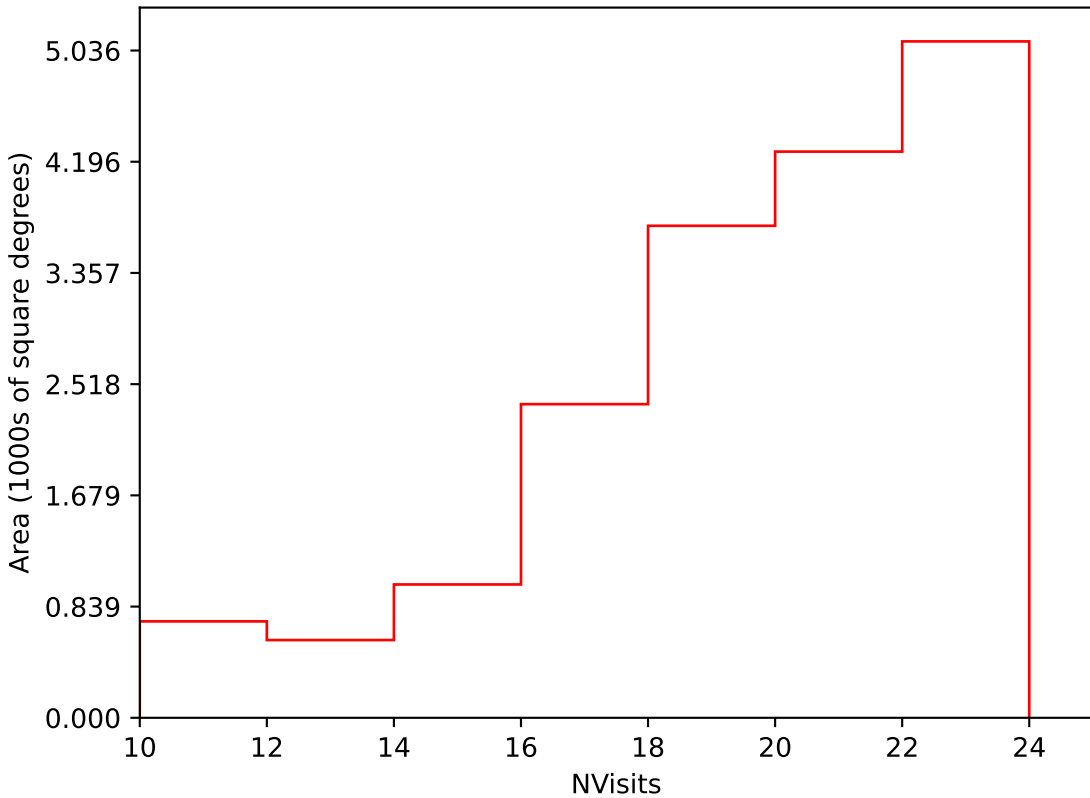
too_elab_r32_d3_giz_v3.4_10yrs Yr 1 i band: NVisits
