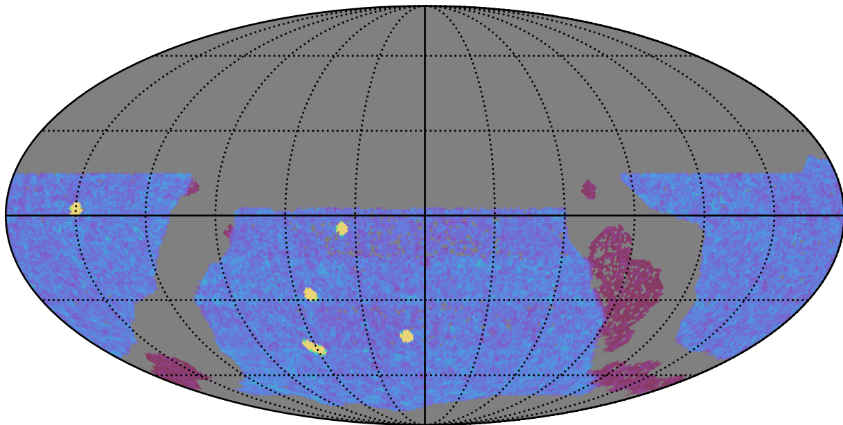
too_elab_r32_d3_giz_v3.4_10yrs WFD y band: NVisits
