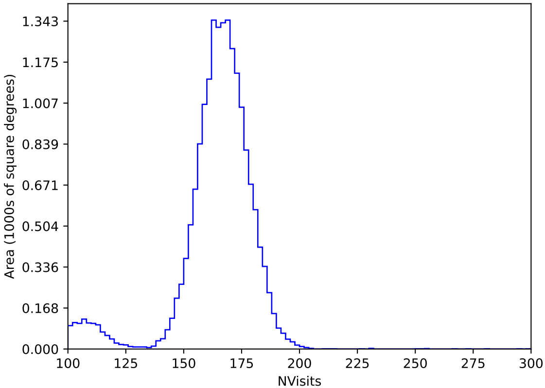
too_elab_r32_d3_giz_v3.4_10yrs WFD y band: NVisits
