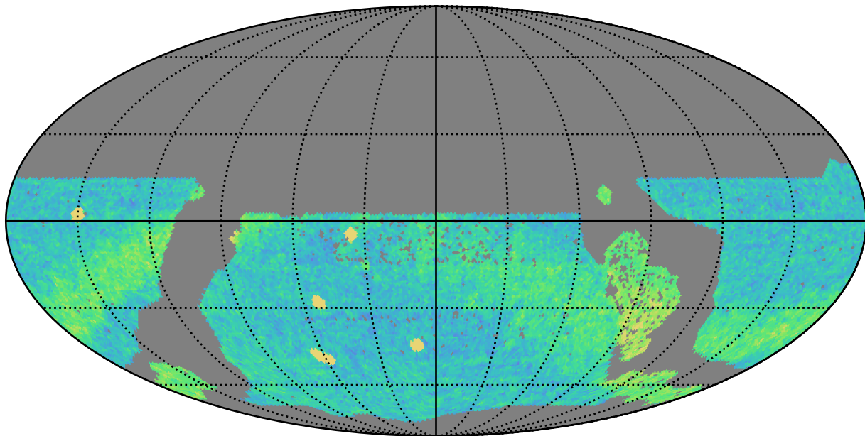
too_elab_r32_d3_giz_v3.4_10yrs WFD r band: NVisits
