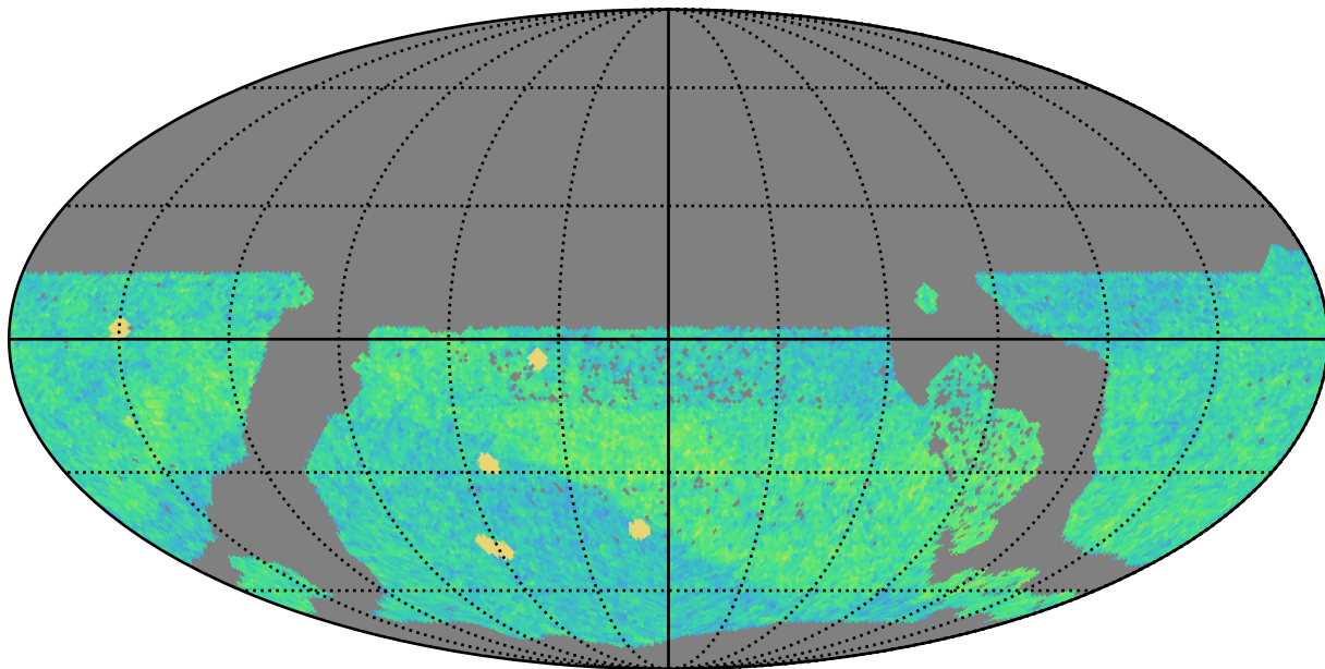
too_elab_r32_d3_giz_v3.4_10yrs WFD i band: NVisits
