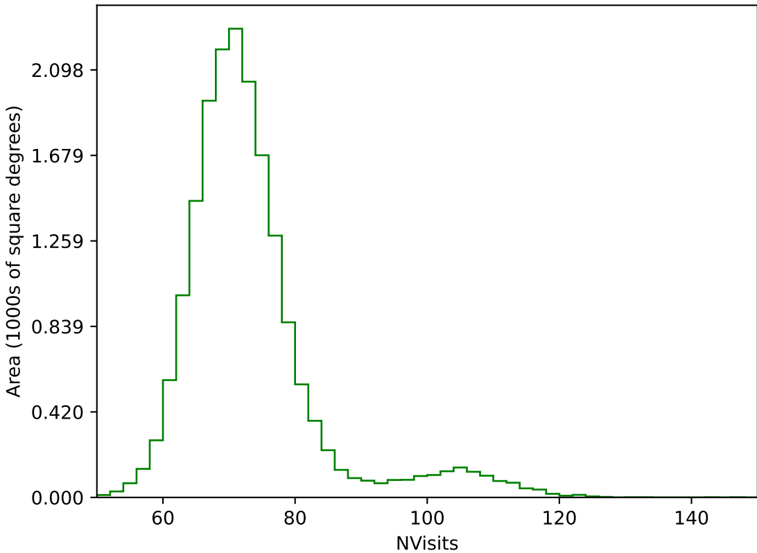
too_elab_r32_d3_giz_v3.4_10yrs WFD g band: NVisits
