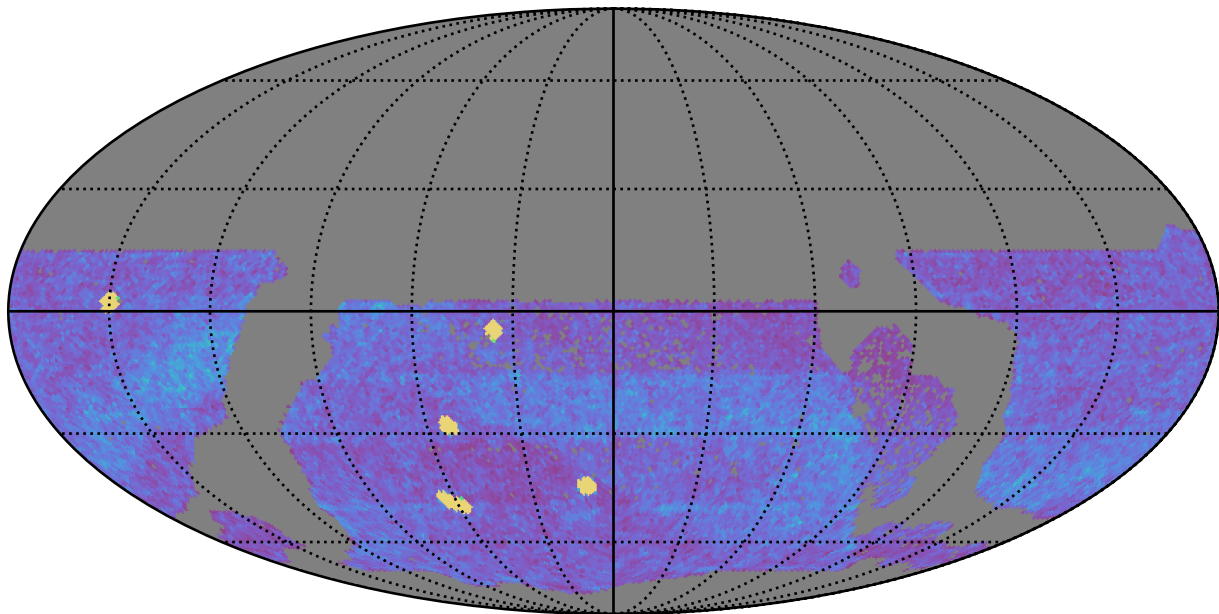
too_elab_r32_d3_giz_v3.4_10yrs WFD all bands: NVisits
