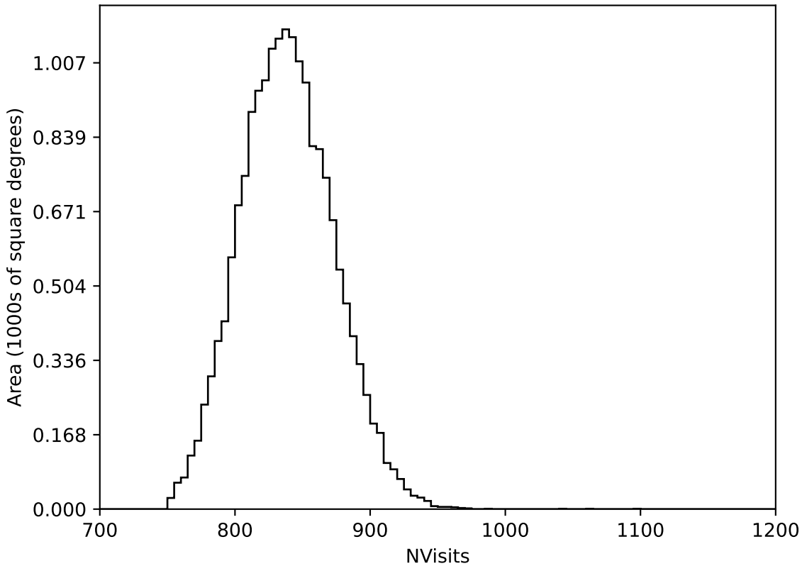
too_elab_r32_d3_giz_v3.4_10yrs WFD all bands: NVisits
