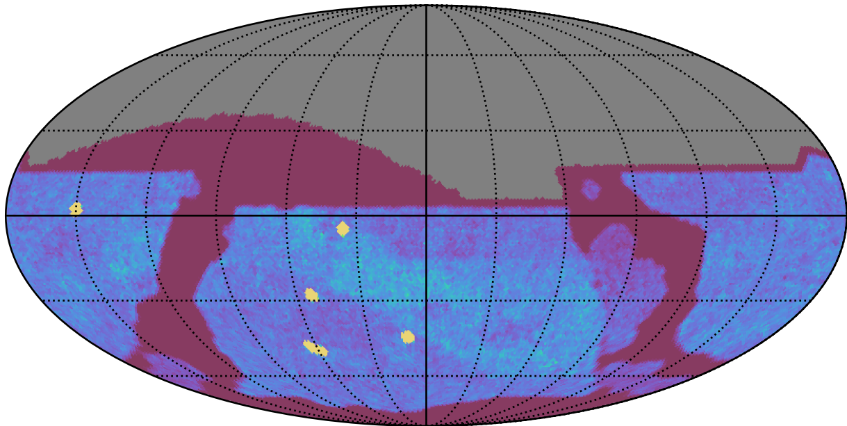
too_elab_r32_d3_giz_v3.4_10yrs All sky z band: NVisits
