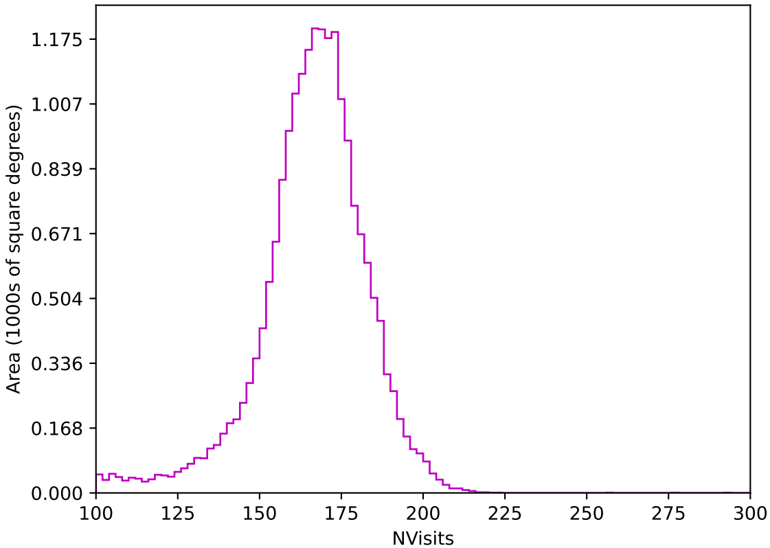
too_elab_r32_d3_giz_v3.4_10yrs All sky z band: NVisits
