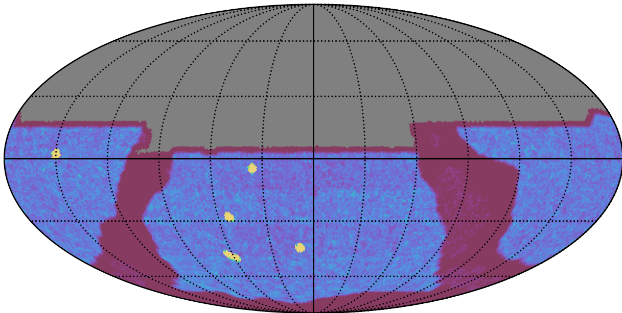
too_elab_r32_d3_giz_v3.4_10yrs All sky y band: NVisits
