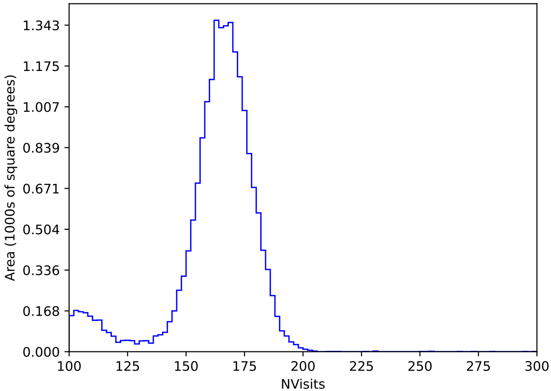
too_elab_r32_d3_giz_v3.4_10yrs All sky y band: NVisits
