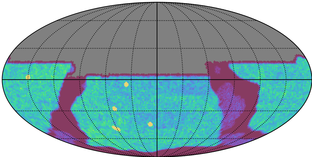
too_elab_r32_d3_giz_v3.4_10yrs All sky u band: NVisits
