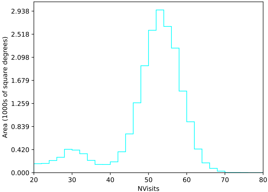
too_elab_r32_d3_giz_v3.4_10yrs All sky u band: NVisits
