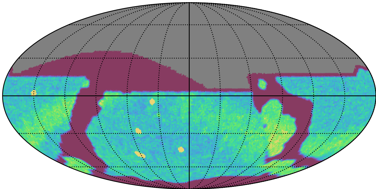
too_elab_r32_d3_giz_v3.4_10yrs All sky r band: NVisits
