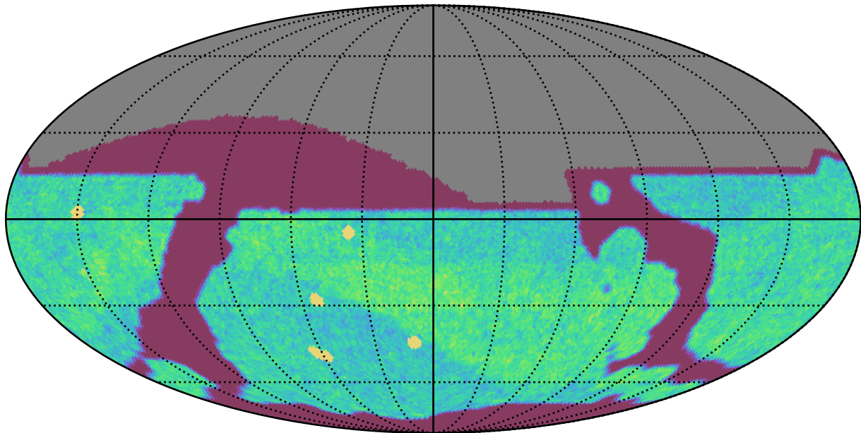
too_elab_r32_d3_giz_v3.4_10yrs All sky i band: NVisits
