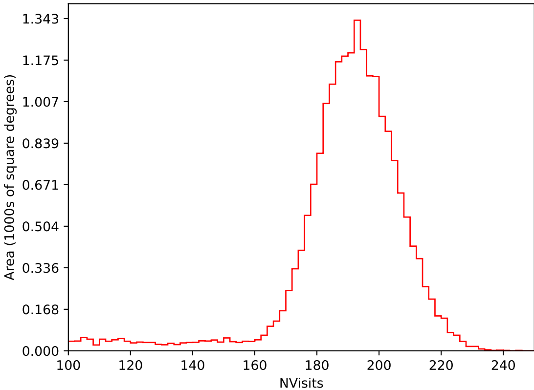
too_elab_r32_d3_giz_v3.4_10yrs All sky i band: NVisits
