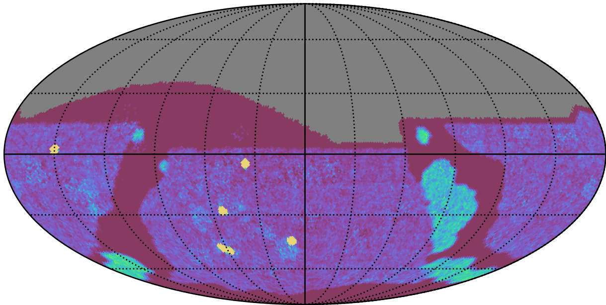
too_elab_r32_d3_giz_v3.4_10yrs All sky g band: NVisits
