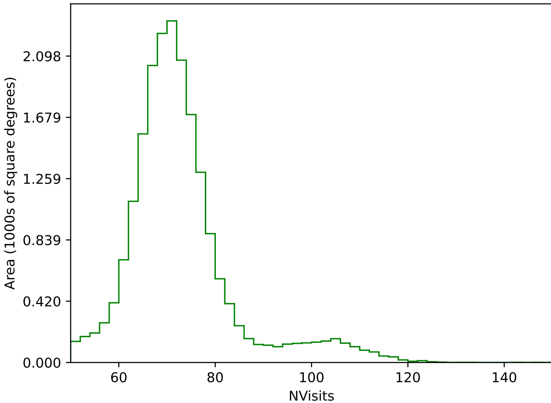
too_elab_r32_d3_giz_v3.4_10yrs All sky g band: NVisits
