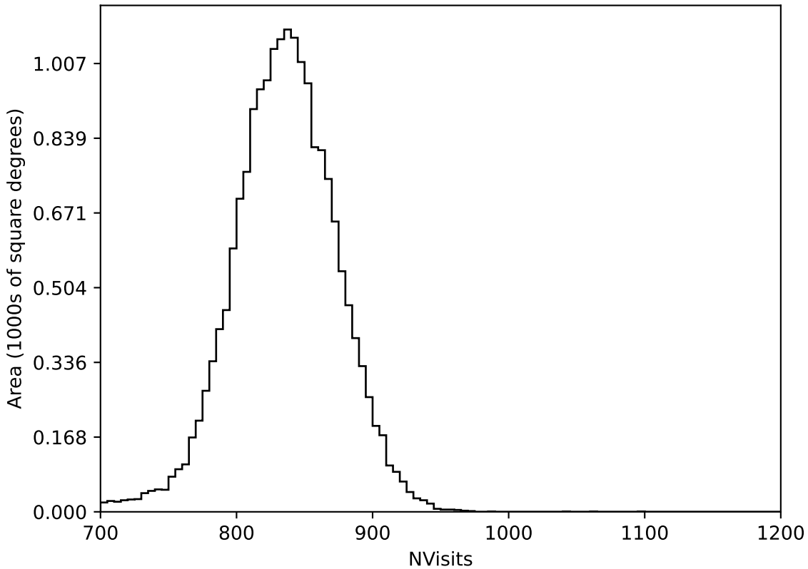
too_elab_r32_d3_giz_v3.4_10yrs All sky all bands: NVisits
