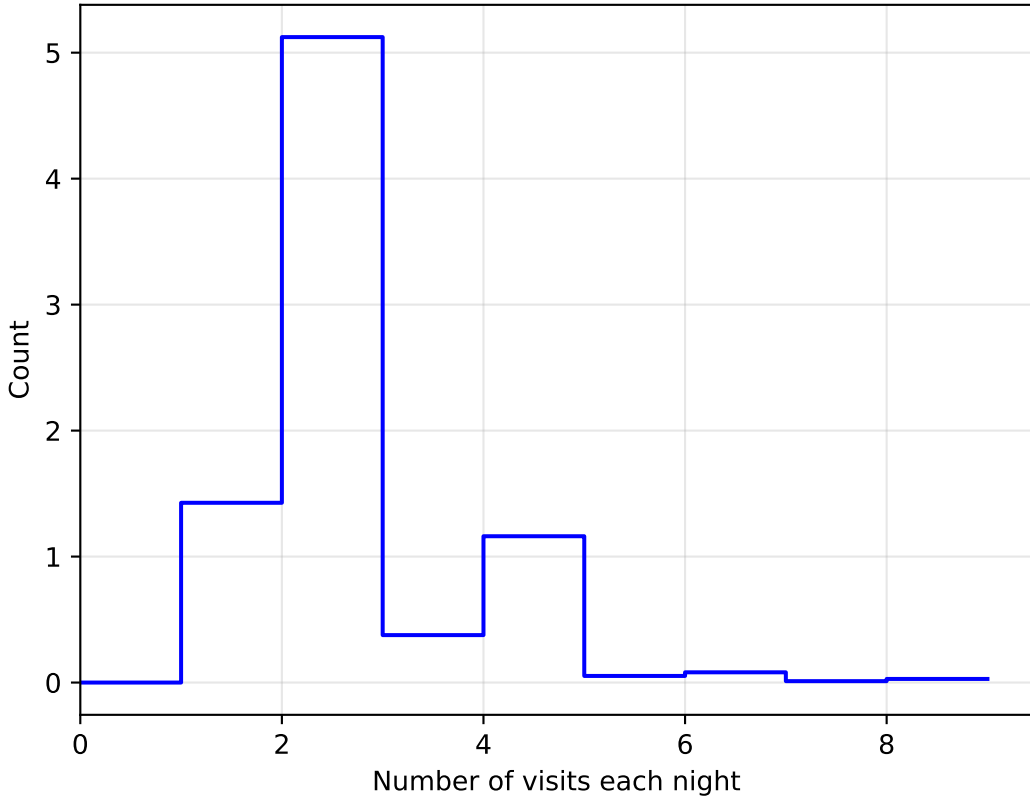
too_elab_r32_d3_giz_v3.4_10yrs WFD: NVisitsPerNight
