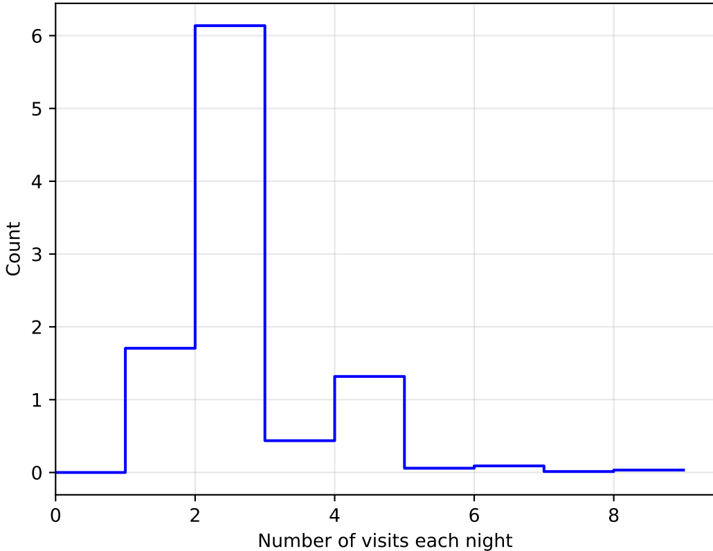
too_elab_r32_d3_giz_v3.4_10yrs All sky: NVisitsPerNight
