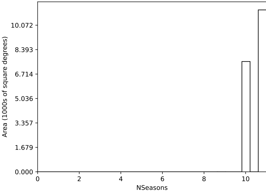
too_elab_r32_d3_giz_v3.4_10yrs WFD all bands: NSeasons
