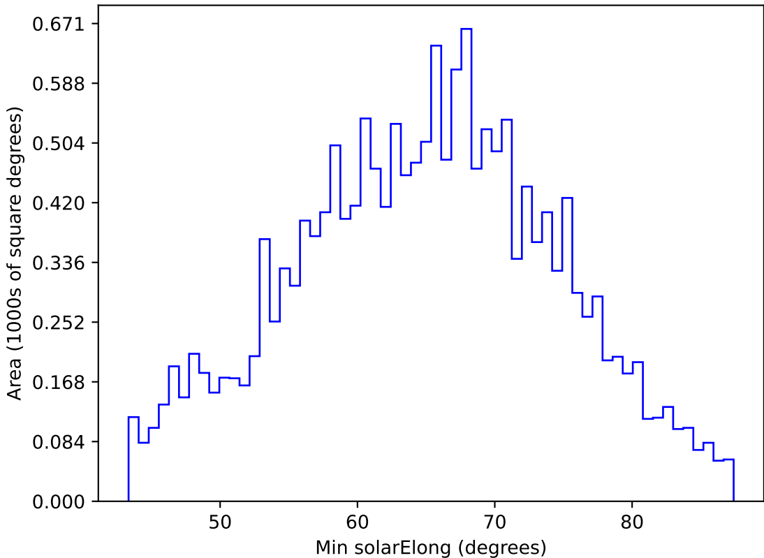
too_elab_r32_d3_giz_v3.4_10yrs WFD y band: Min solarElong
