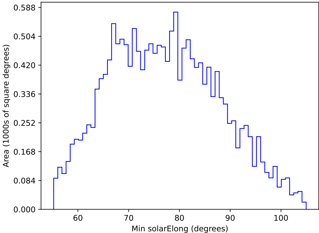
too_elab_r32_d3_giz_v3.4_10yrs WFD u band: Min solarElong
