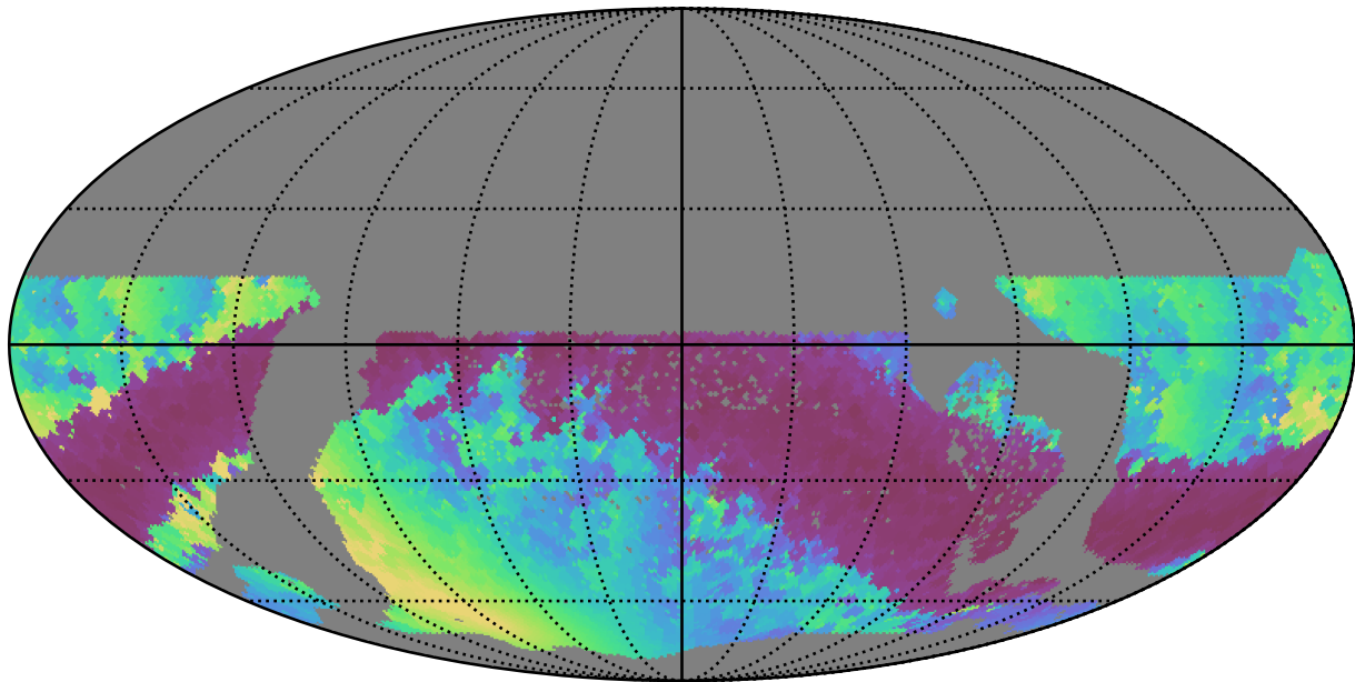
too_elab_r32_d3_giz_v3.4_10yrs WFD r band: Min solarElong
