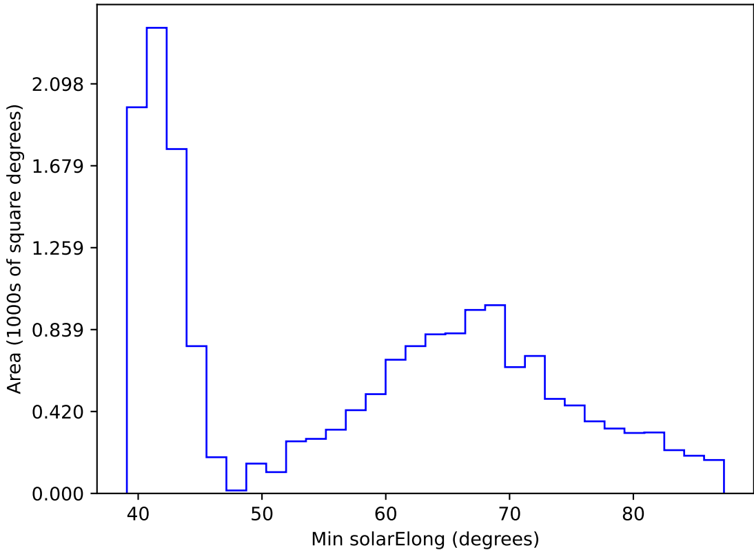
too_elab_r32_d3_giz_v3.4_10yrs WFD r band: Min solarElong
