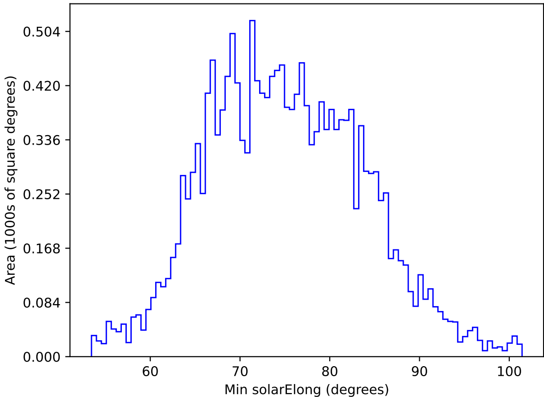
too_elab_r32_d3_giz_v3.4_10yrs WFD g band: Min solarElong
