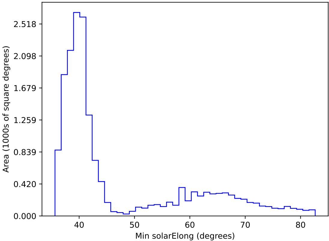
too_elab_r32_d3_giz_v3.4_10yrs WFD all bands: Min solarElong
