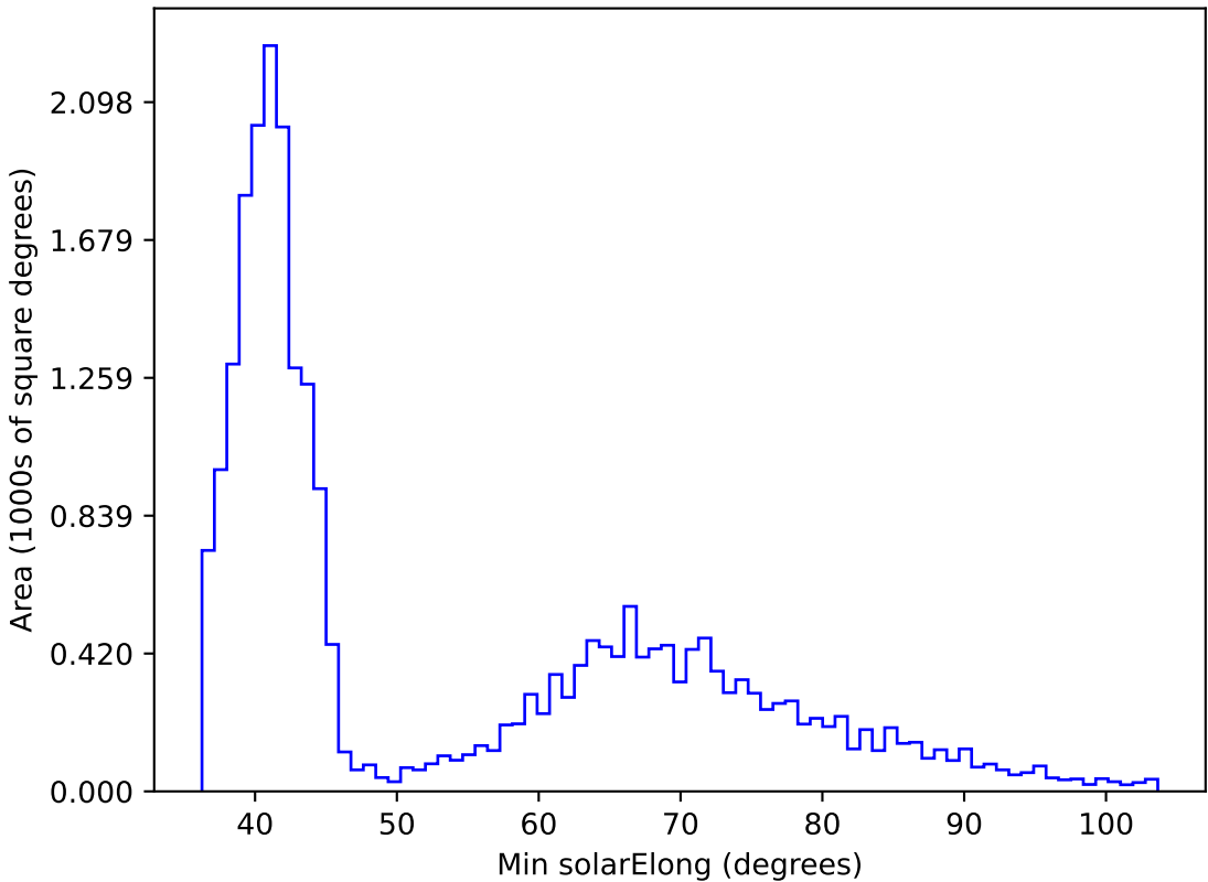
too_elab_r32_d3_giz_v3.4_10yrs All sky z band: Min solarElong
