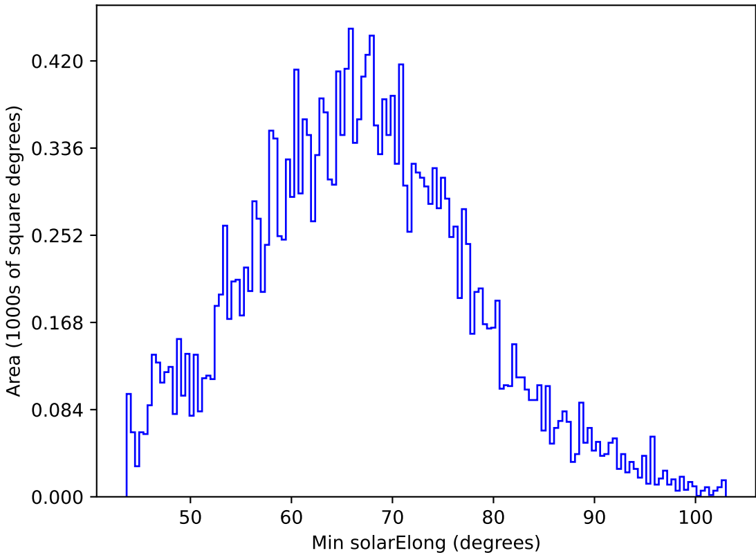
too_elab_r32_d3_giz_v3.4_10yrs All sky y band: Min solarElong
