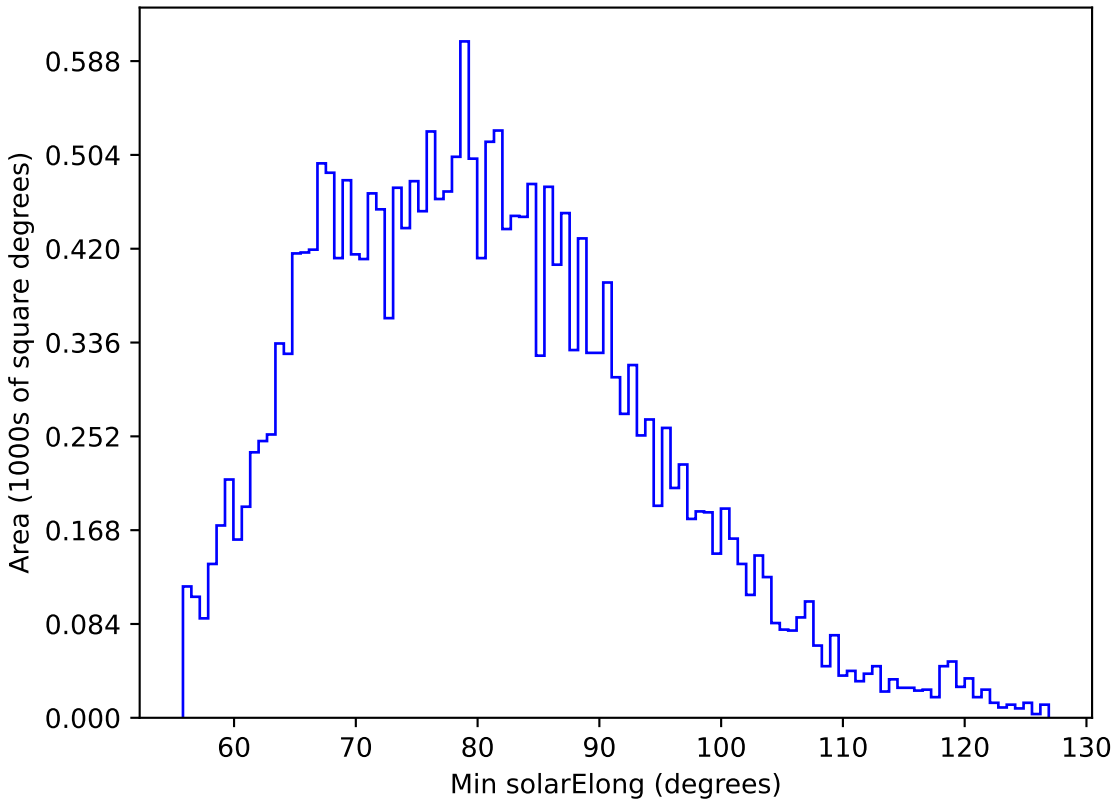
too_elab_r32_d3_giz_v3.4_10yrs All sky u band: Min solarElong
