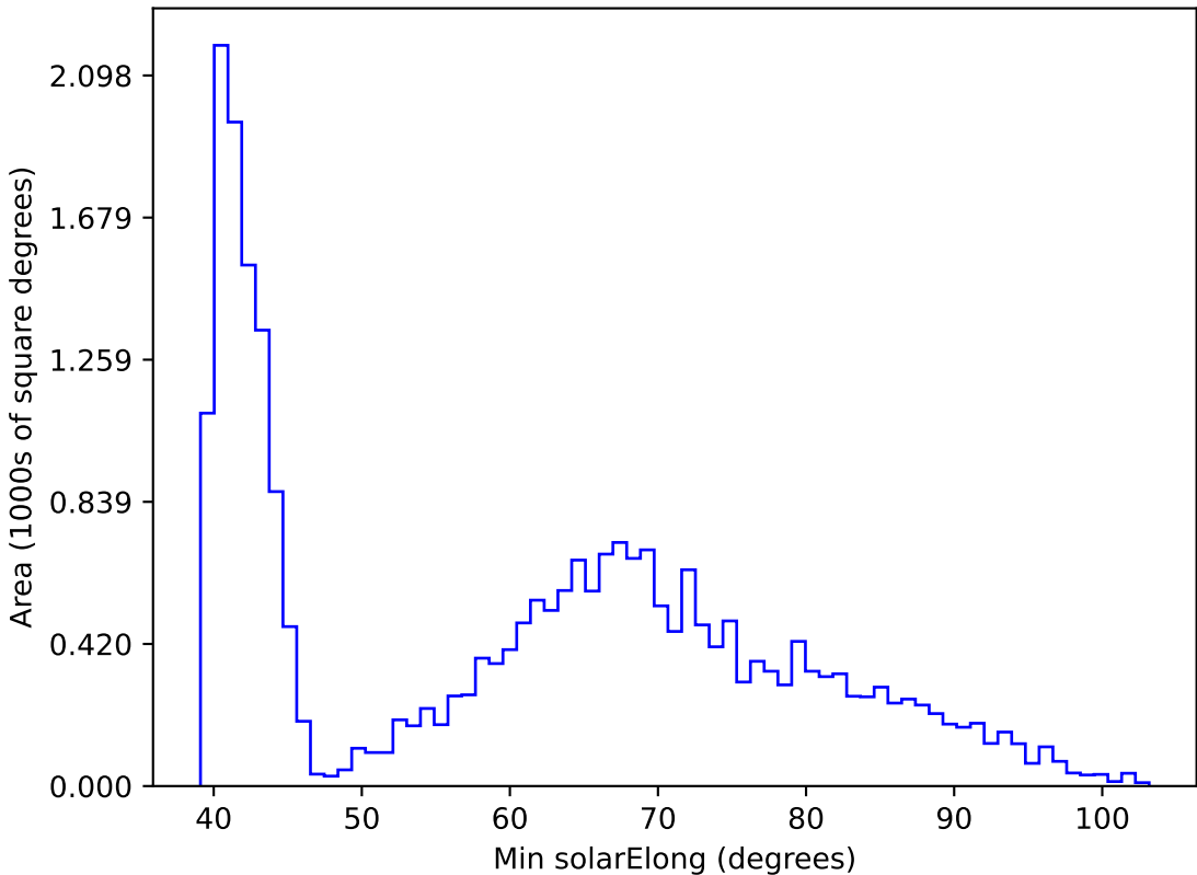
too_elab_r32_d3_giz_v3.4_10yrs All sky r band: Min solarElong
